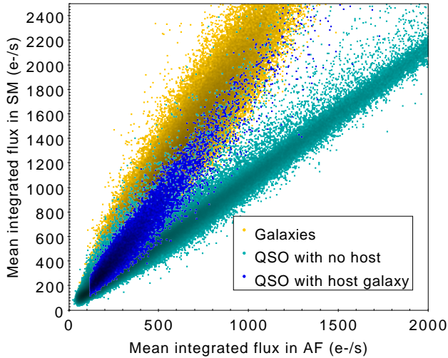
Fig. 2. Comparison of the flux collected in the AF and SM windows in the Gaia focal plane for quasars (with and without a detected host galaxy in Gaia ) and for galaxies. Objects with an extension detectable by Gaia lie above the turquoise diagonal of quasars with no host galaxy.
