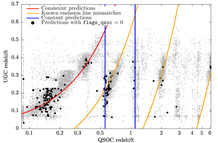
Fig. 21. Comparison between the UGC and QSOC redshifts. Grey dots correspond to all redshifts in common between the two tables, while black dots are restricted to those with flags\_qsoc = 0 , which corresponds to a higher reliability subset. The red curve denotes identical predictions in the two modules. Yellow curves highlight mismatches between common quasar or AGN emission lines, as explained in Delchambre et al. (2023), while the blue vertical lines show constant predictions by QSOC.
